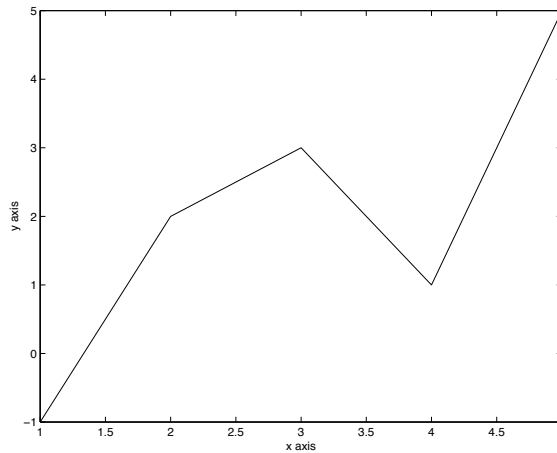
Figure 1: Plot \mathbf{x} versus \mathbf{y} for the vectors \mathbf{x} = (1, 2, 3, 4, 5) and \mathbf{y} = (-1, 2, 3, 1, 5) .
