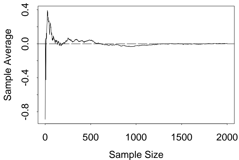
Sn/n vs. n, N(0,1) Data
