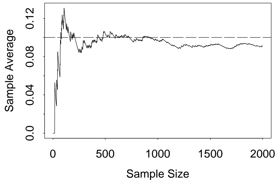
Sn/n vs. n, Bin(1,.1) Data
