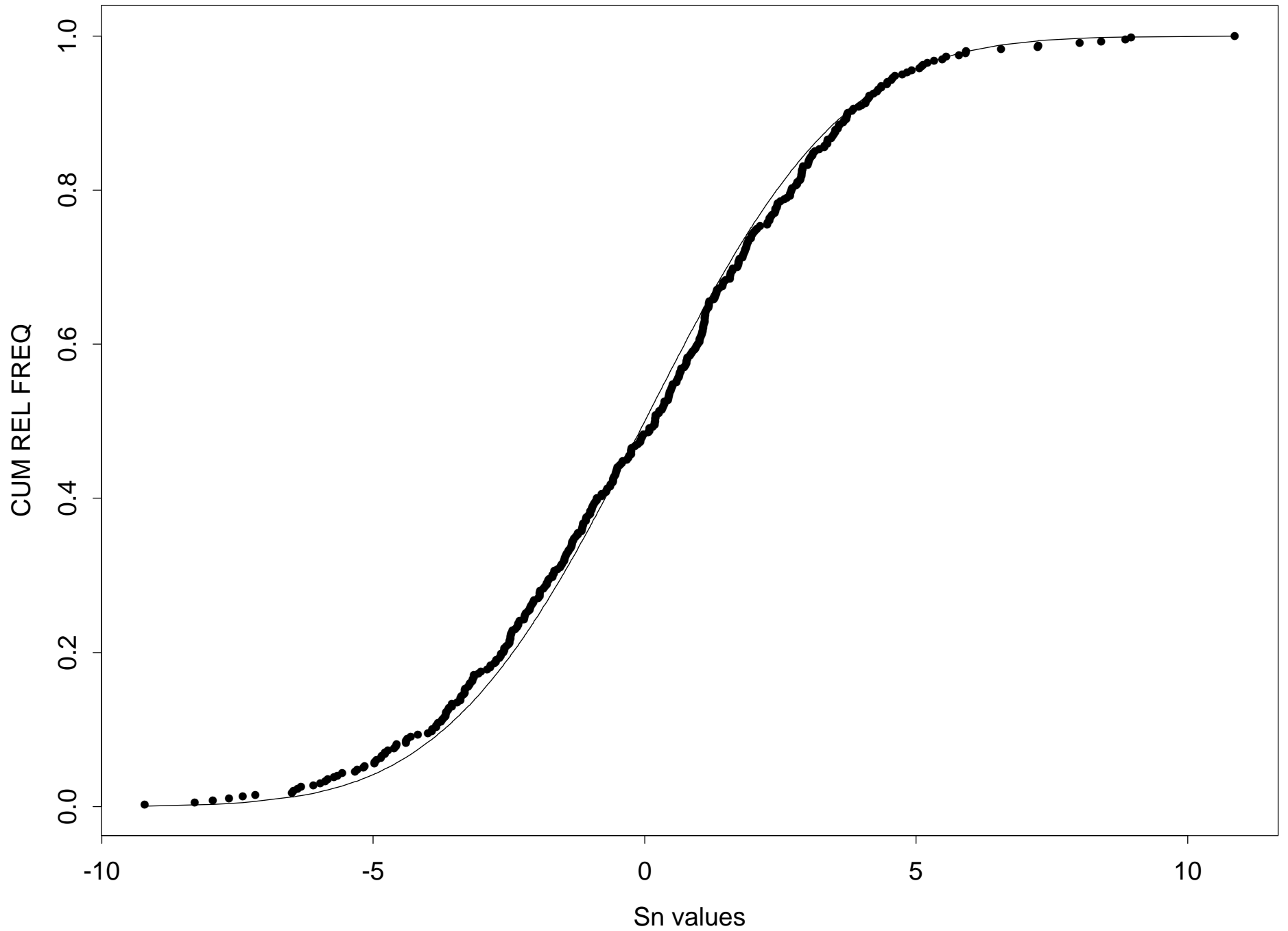
Empirical Dist Fcn of S_n(i) With Overlaid Normal(0,100/12) CDF
