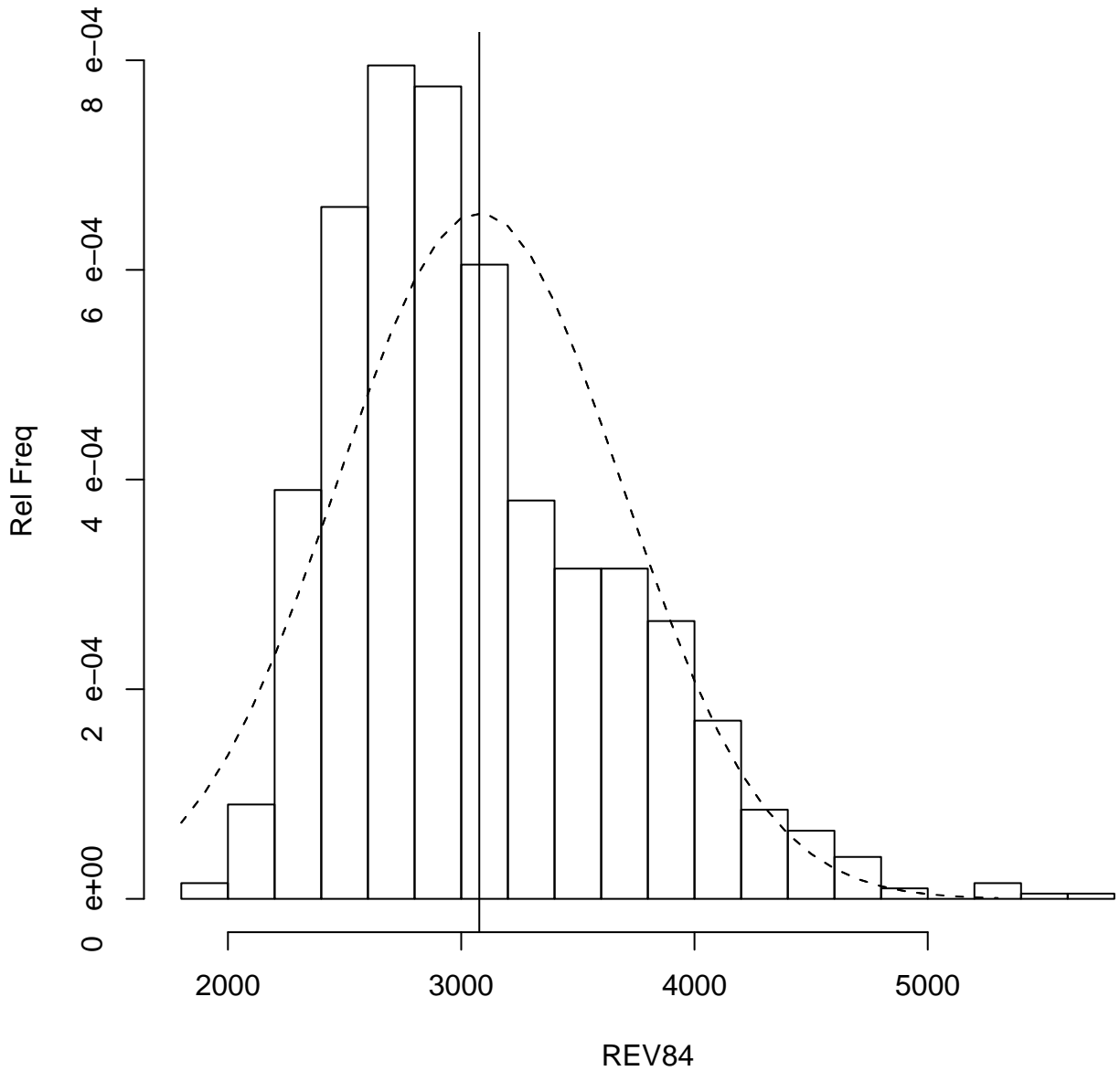
Histogram of SRS Means from Mu284, n=50
