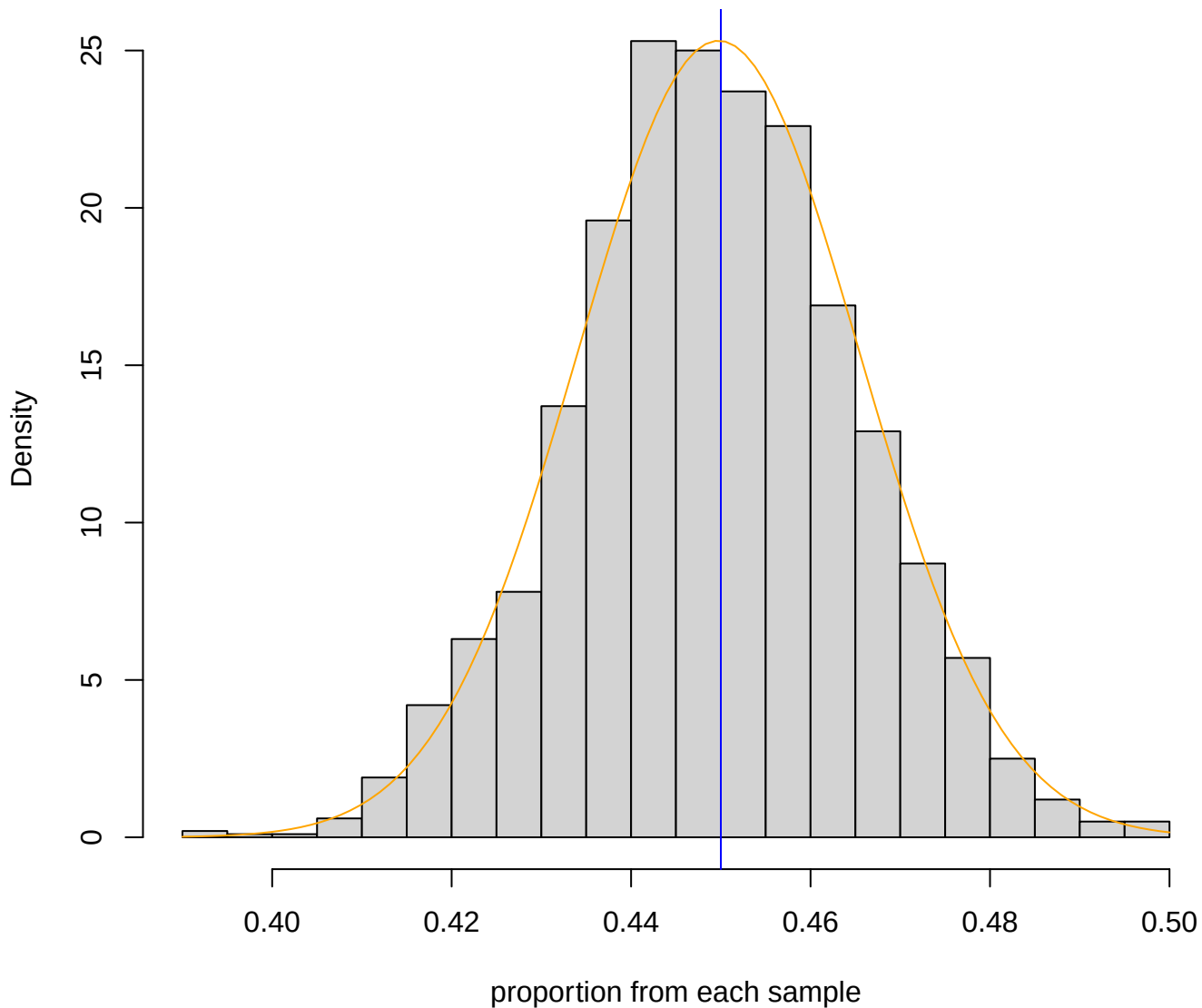
Histogram of sample proportions from 2000 sample draws SRS samples of n=1000 from N=100,000 , with true prop.=0.45
