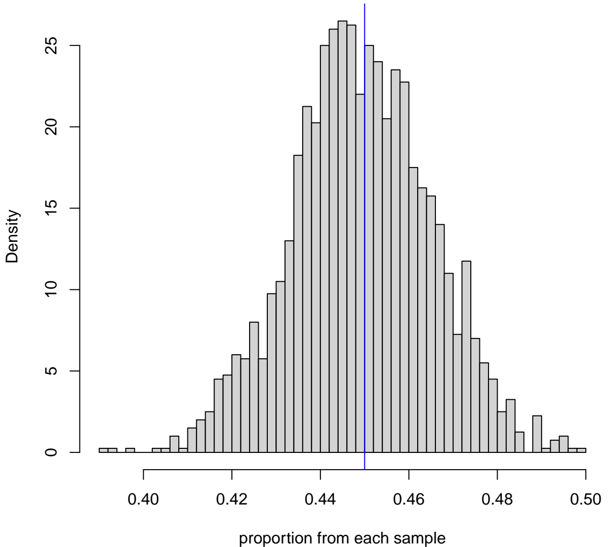
Histogram of sample proportions from 2000 sample draws SRS samples of n=1000 from N=100,000 , with true prop.=0.45
