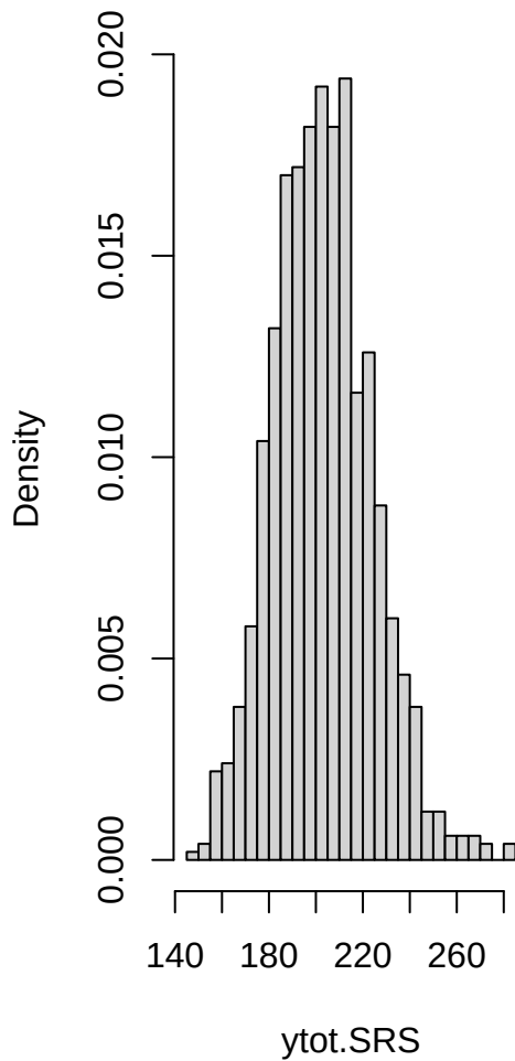
SRS Hist
