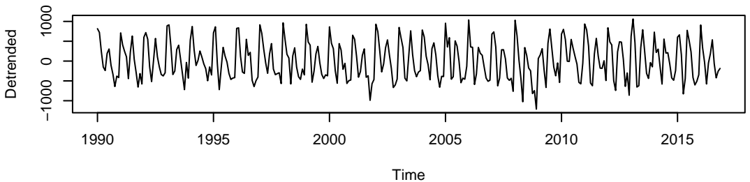
1-Step-Ahead fitted unemp minus trend from 'seasonal' package
