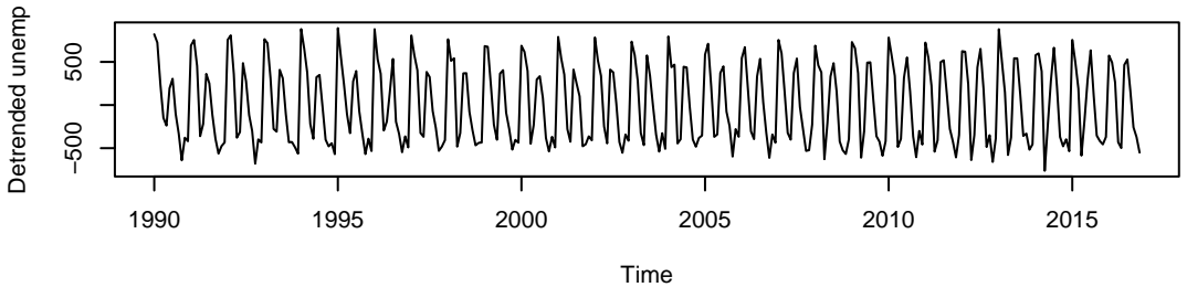
unemp minus trend from package 'seasonal'
