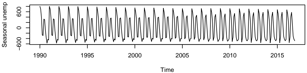
Seasonal component of unemp from package 'seasonal'
