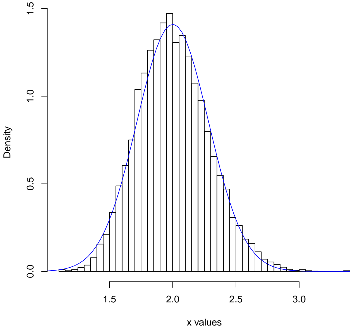
10,000 sample means of size 25, Gamma(2,1) data Overlaid with blue Normal density curve from CLT
