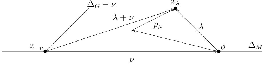
FIGURE 1. The broken path p_\mu from o to x_\lambda is an LS path of type \mu . Then the Littellmann bigon with the sides p_\mu and \overline{ox_\lambda} yields a Littellmann triangle with the geodesic sides \overline{x_{-\nu}o} , \overline{x_{-\nu}x_\lambda} and the broken side p_\mu .
